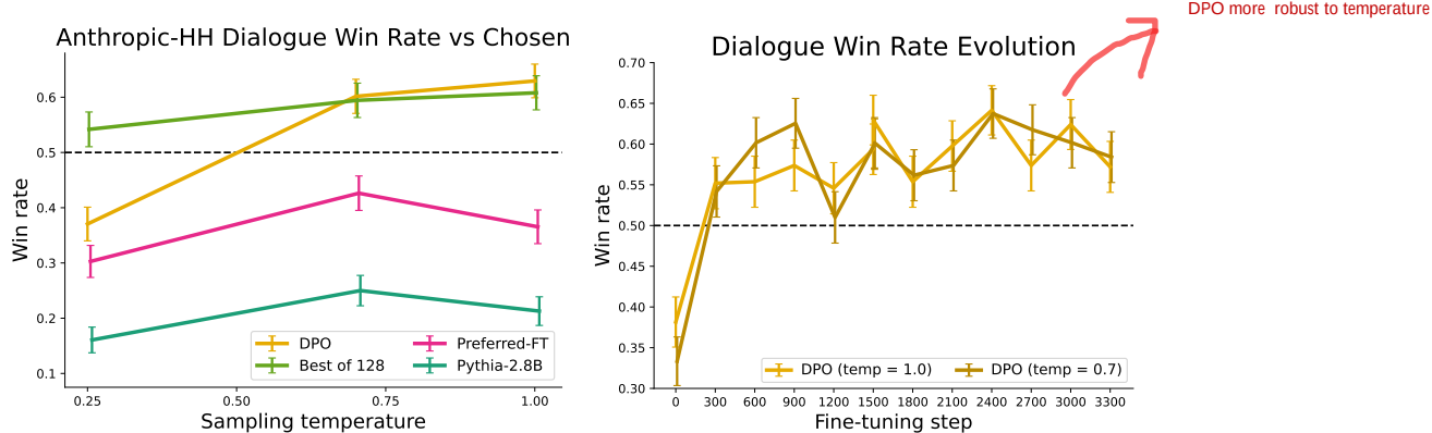
Figure 3: Left. Win rates computed by GPT-4 for Anthropic-HH one-step dialogue; DPO is the only method that improves over chosen summaries in the Anthropic-HH test set. Right. Win rates for different sampling temperatures over the course of training. DPO’s improvement over the dataset labels is fairly stable over the course of training for different sampling temperatures.
